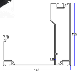
Povezani pravi oluk Straight Gutter Connected
