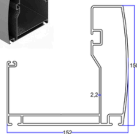
Povezani veliki oluk Large Gutter Connected
