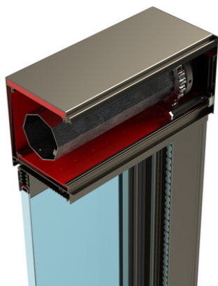
Izolovana kutija Insulated box
