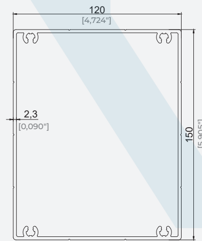
120x150 Profil Stuba 120x150 Pillar Profile
