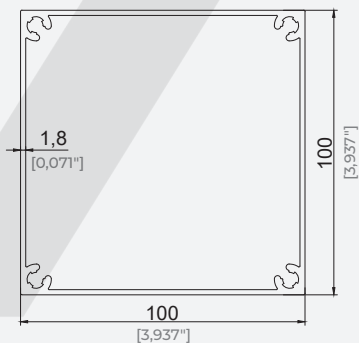
100x100 Profil Stuba 100x100 Pillar Profile
