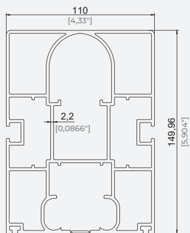
110x150 Šine Profil 110x150 Rail Profile
