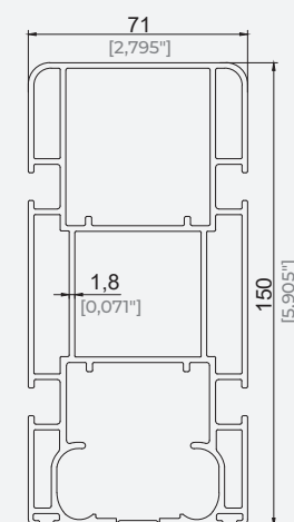
71x150 Šine Profil 71x150 Rail Profile
