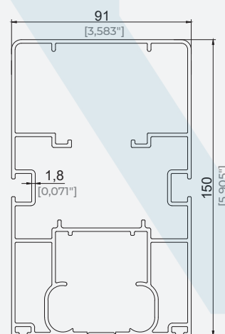
91x150 Šine Profil 91x150 Eco Rail Profile
