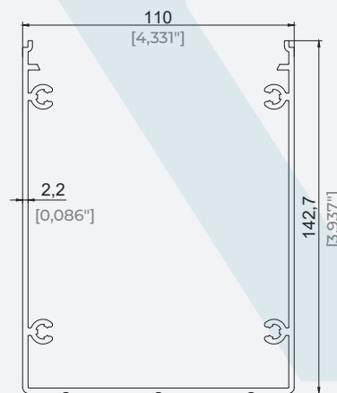
110x142,7 Profil Stuba-1 110x142,7 Pillar Main Profile
