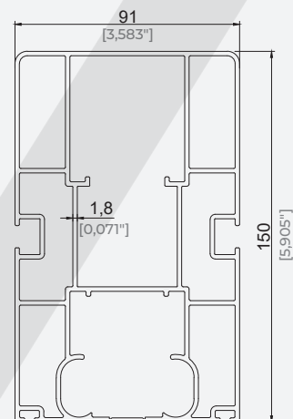
91x150 Šine Profil 91x150 Rail Profile
