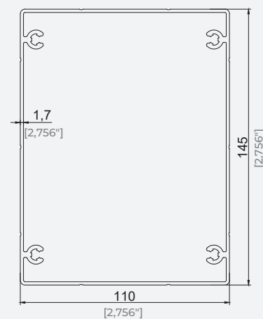
110x145 Profil Stuba 110x145 Pillar Profile
