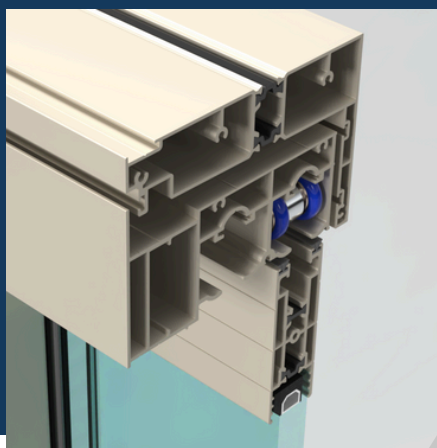
Detalj gornjeg dela Upper case detail
