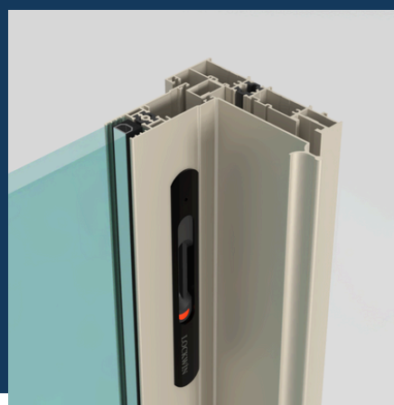
Detalj završnog profila Finish profile detail
