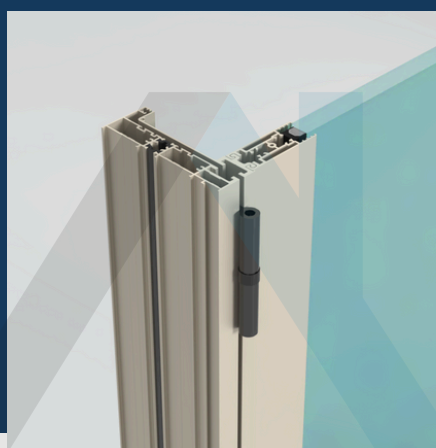
Detalj kliznih vrata Sliding Door detail
